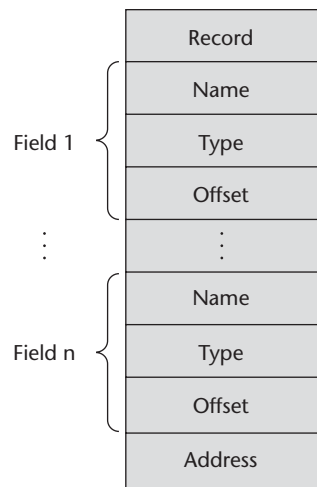
Figure 6.7 A compile-time descriptor for a record
