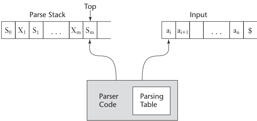
Figure 4.4 The structure of an LR parser
